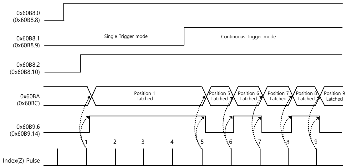
Index Pulse Trigger Mode (0x60B8.2=1, 0x60B8.10=1):
