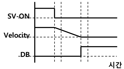
Free Run Stop 후 Hold
