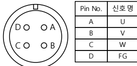
<Power Connector>
