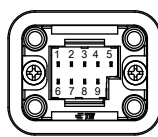
<Encoder Connector 핀 배열>
