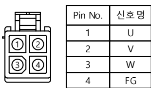
<Power Connector>
