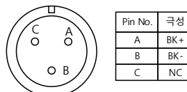
<Brake Connector>
