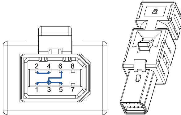
2069577-1(Tyco Electronics)
