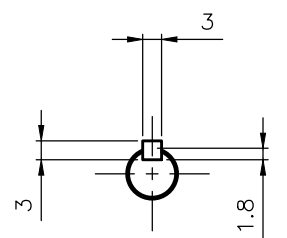
<Shaft Dimensions>
