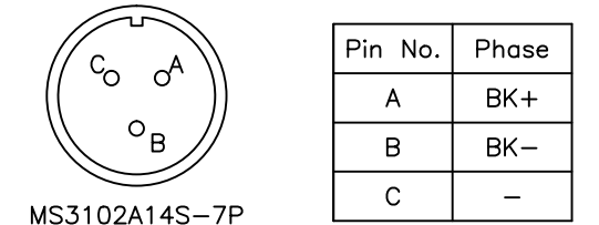
<Brake Connector 핀 배열>
