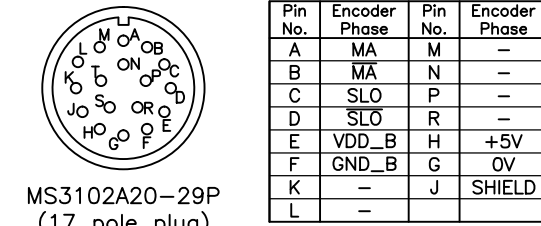
<Encoder Connector 핀 배열>
