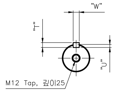
<Shaft Dimensions>
