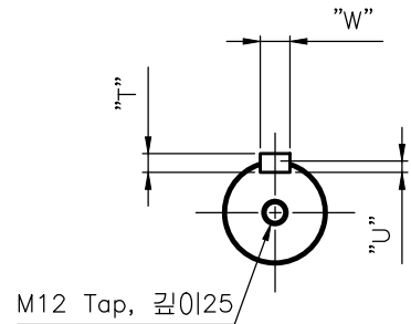
<Shaft Dimensions>
