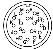
<Encoder Connector 핀 배열>
